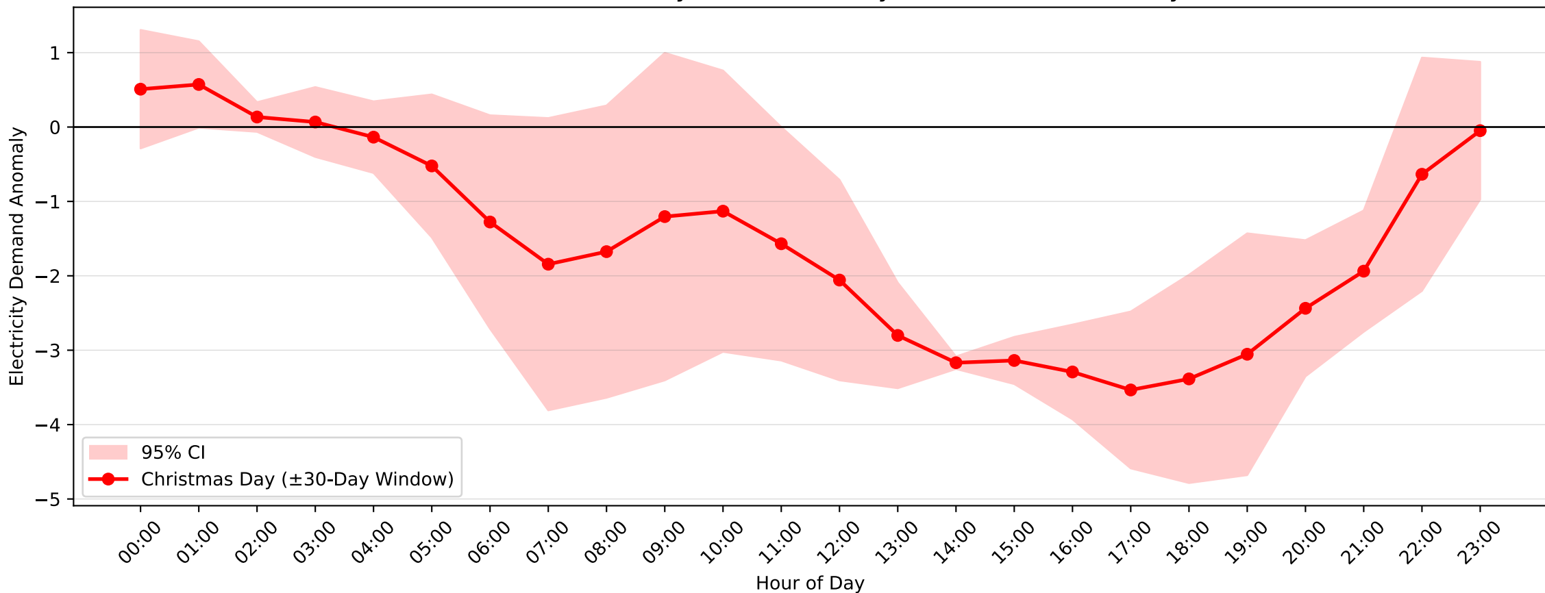
Blakehurst Demand Anomaly: Christmas Day (2005-2006, \pm 30 -Day Window)
