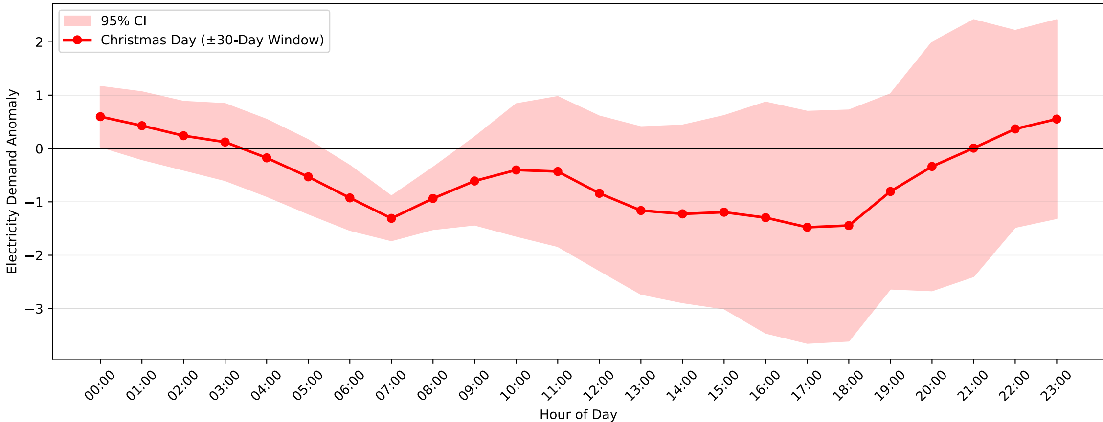
Blakehurst Demand Anomaly: Christmas Day (2010-2011, \pm 30 -Day Window)
