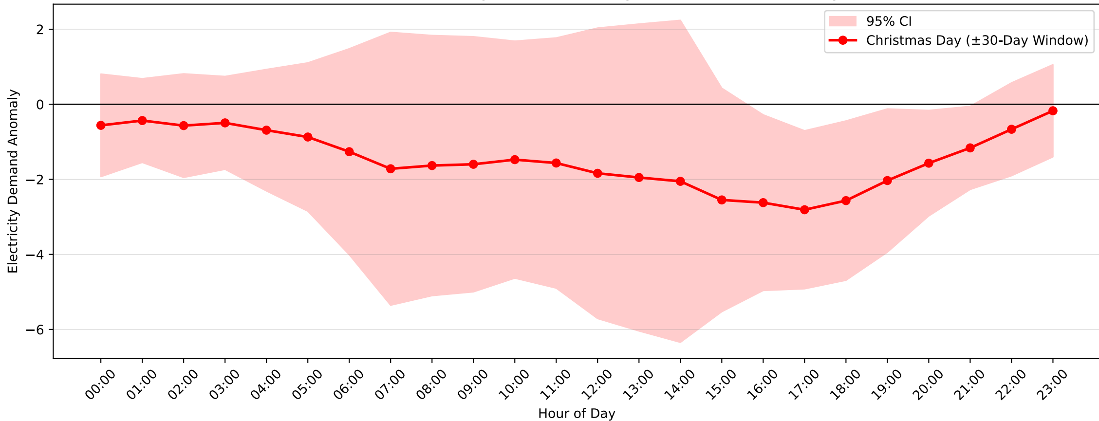
Blakehurst Demand Anomaly: Christmas Day (2009–2010, \pm 30 -Day Window)
