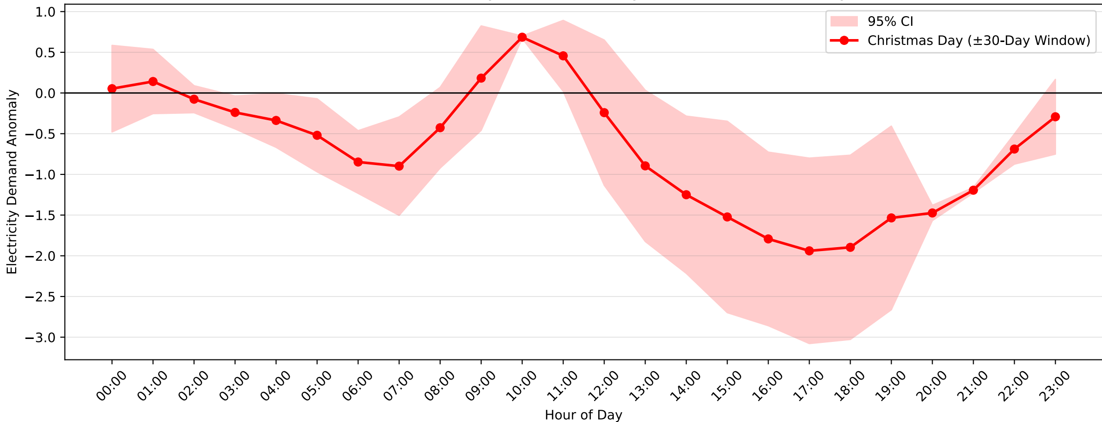
Blakehurst Demand Anomaly: Christmas Day (2015–2016, \pm 30 -Day Window)
